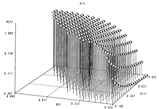
Figure 4: The reaction of the double corrected correlation to changes in \rho[x,y], \rho_{tly}; K = 4 .
