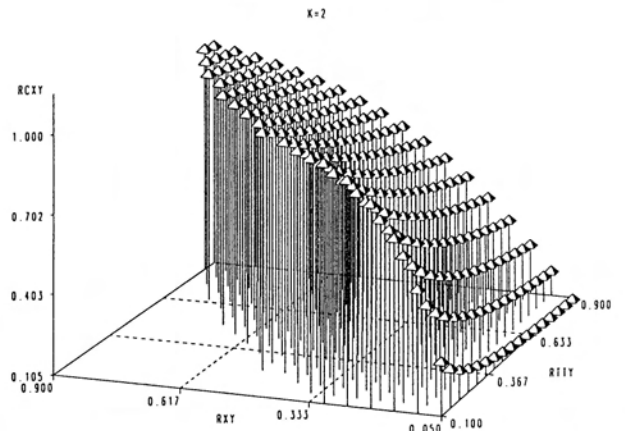
Figure 2: The reaction of the double corrected correlation to changes in \rho[x,y], \rho_{tly}; K = 2 .
