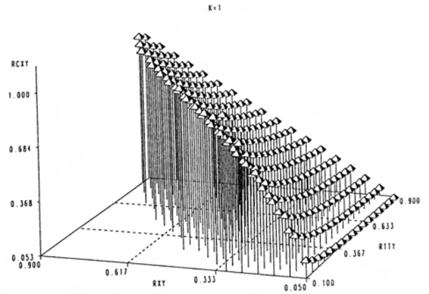
Figure 1: The reaction of the double corrected correlation to changes in \rho[x,y], \rho_{tly}; K = 1 .
