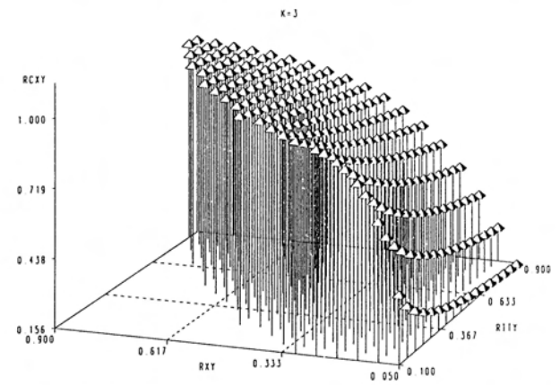
Figure 3: The reaction of the double corrected correlation to changes in \rho[x,y], \rho_{tly}; K = 3 .
